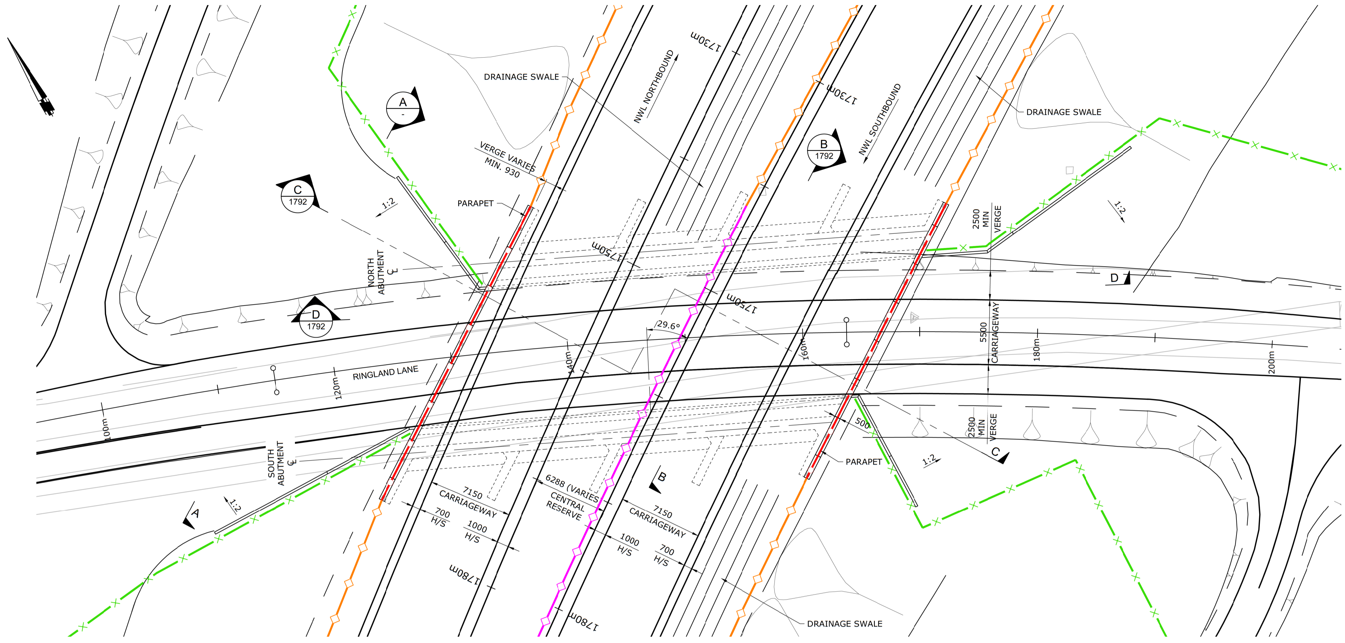
PLAN 1:200
